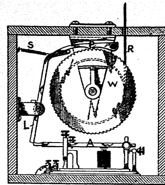
HOW THE BALL IS DROPPED A rope, R , runs up through a flag-staff, out at top, down to ball at base; windlass, W , lifts the ball to top of pole; Observatory clock sends a current through magnet, M , by which armature, A , is instantly lowered; lever, L , held back by resting against end of armature, is now freed; spring, S , jerks it forward, knocks pawl, P , out of ratchet and ball comes down.
